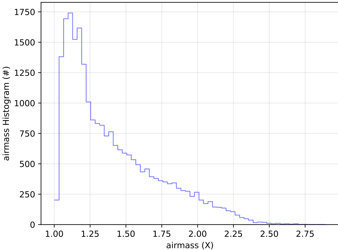
all_long_v3.4_10yrs Yr 1 g band: airmass Histogram
