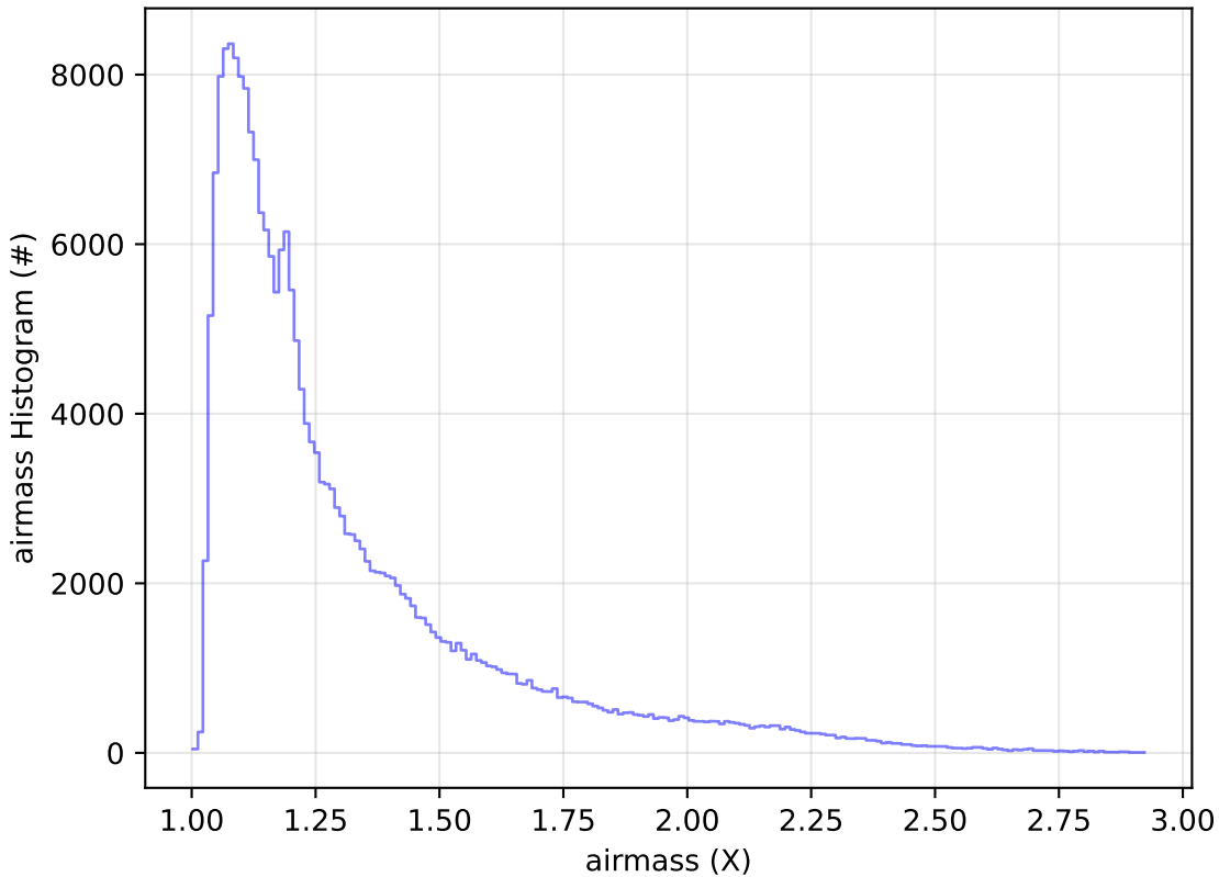
all_long_v3.4_10yrs Yr 1 all bands: airmass Histogram
