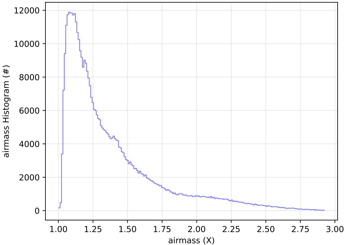
all_long_v3.4_10yrs WFD z band: airmass Histogram
