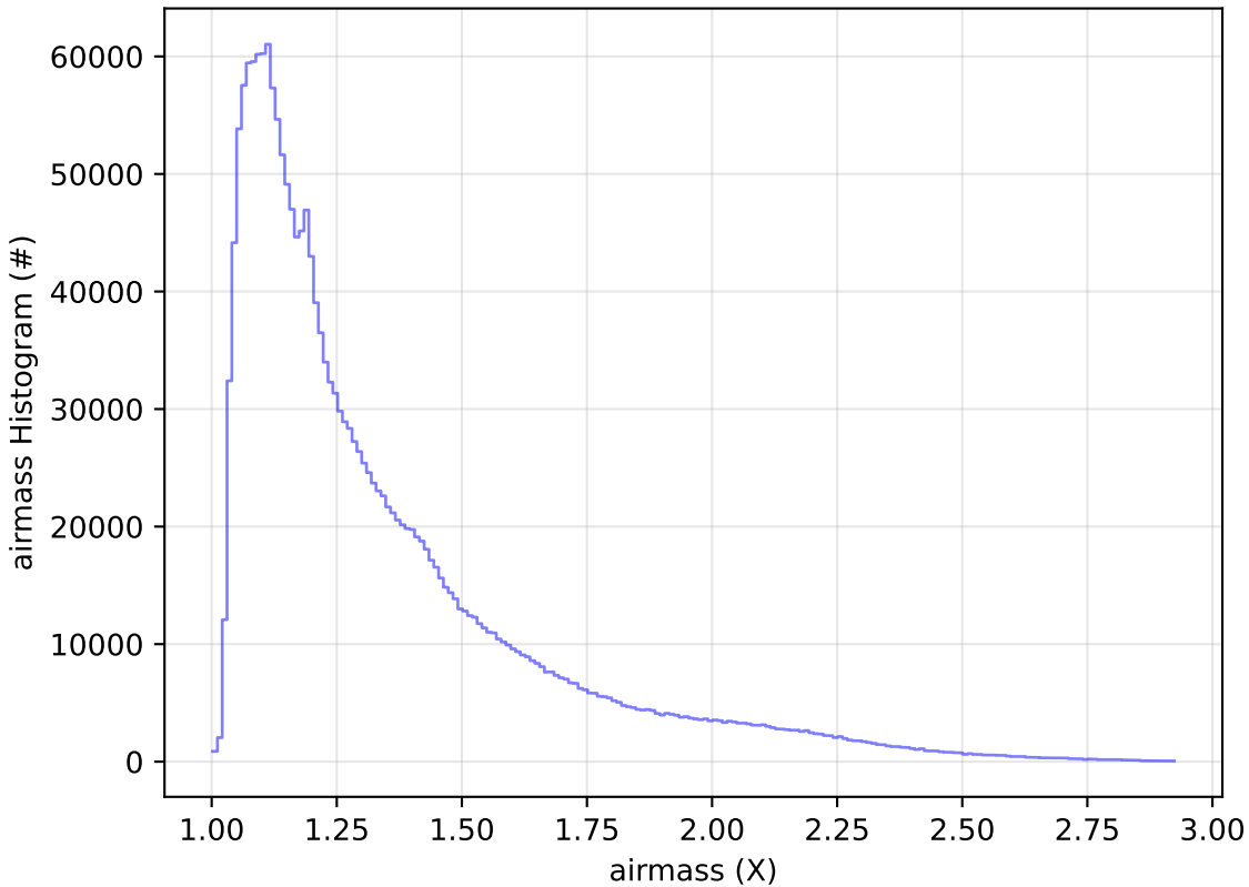
all_long_v3.4_10yrs WFD all bands: airmass Histogram
