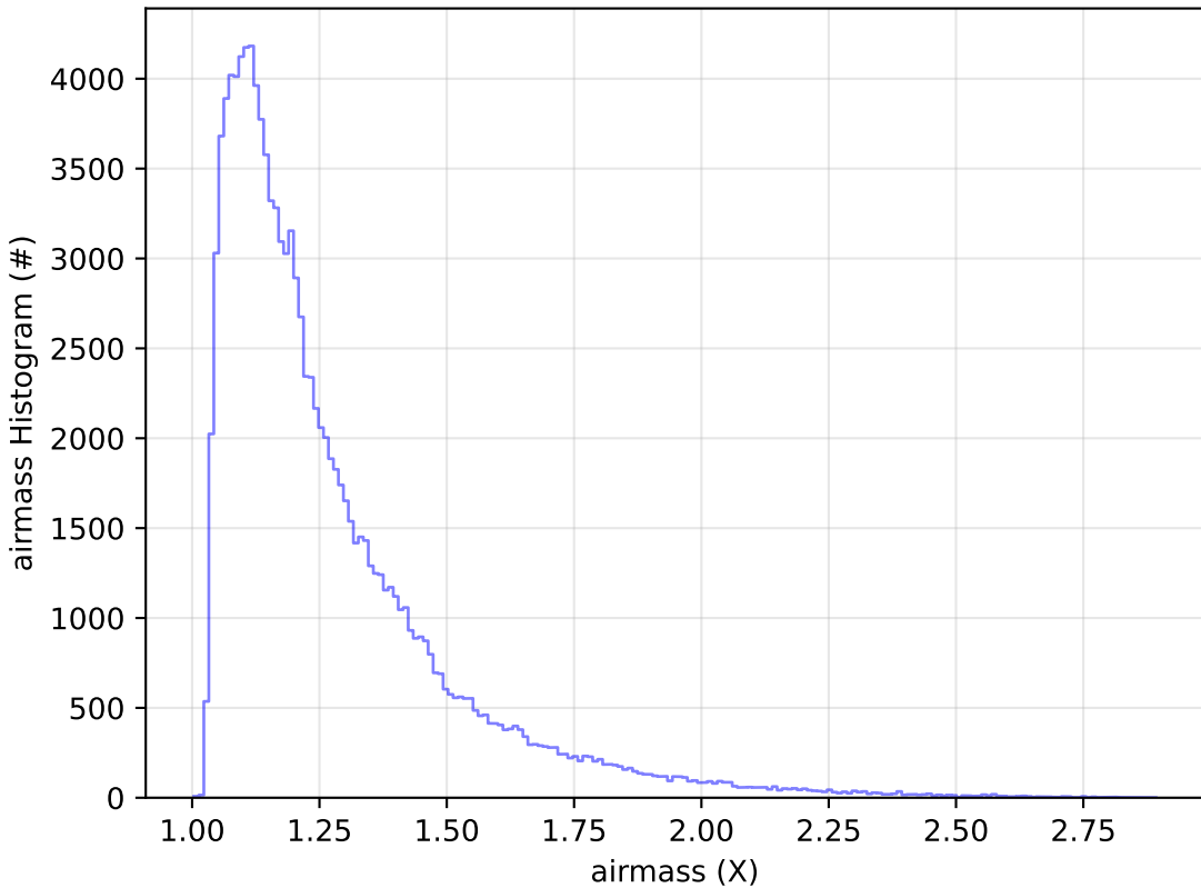
all_long_v3.4_10yrs All sky u band: airmass Histogram
