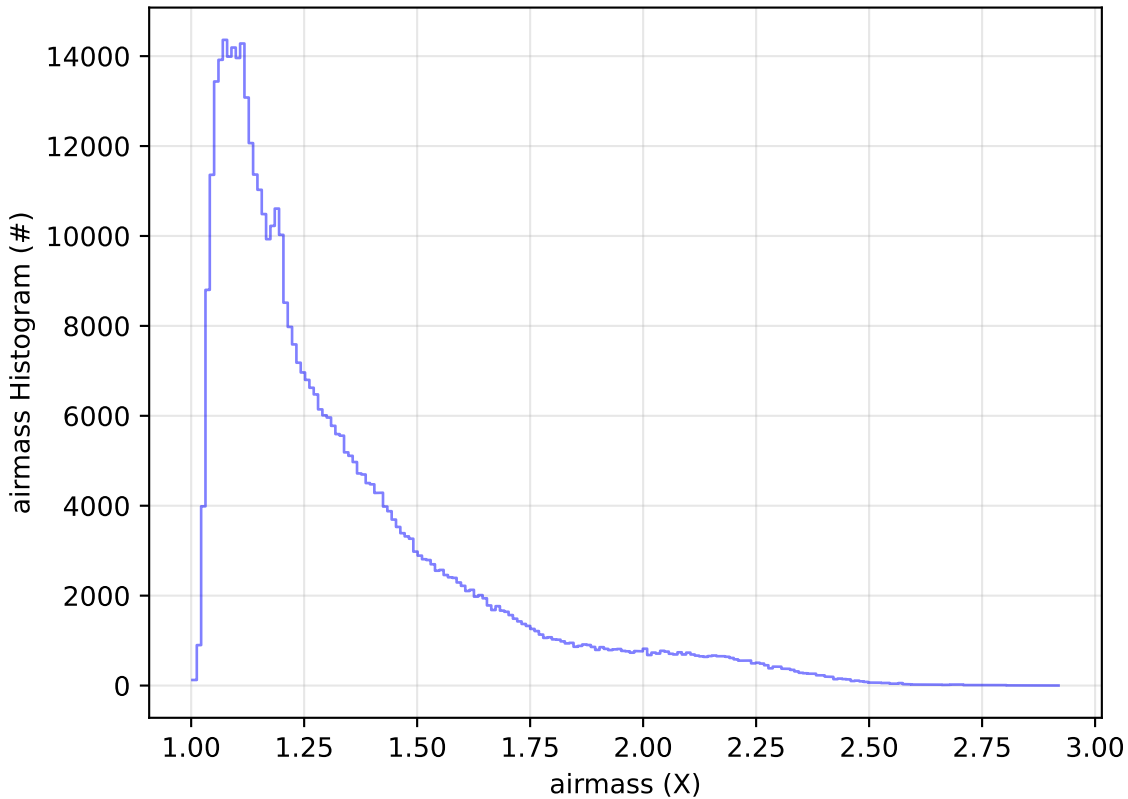
all_long_v3.4_10yrs All sky r band: airmass Histogram
