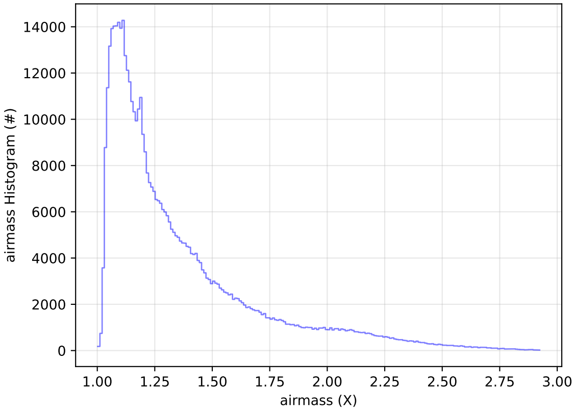
all_long_v3.4_10yrs All sky i band: airmass Histogram
