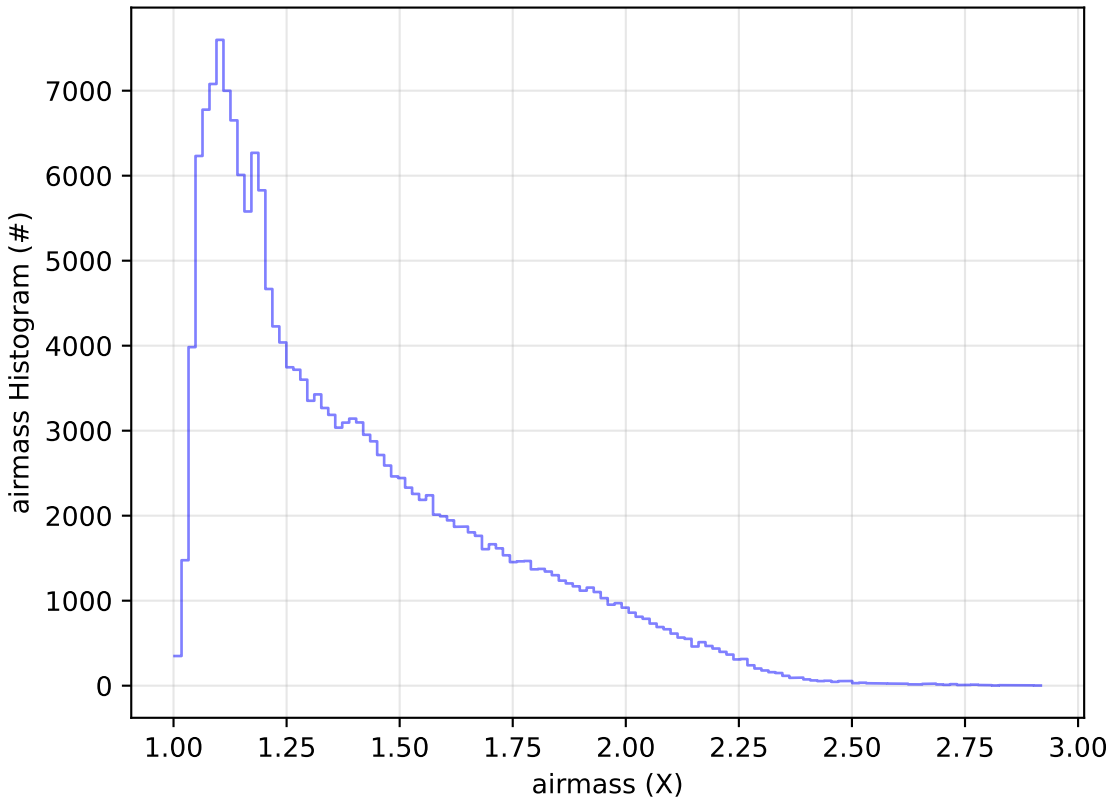
all_long_v3.4_10yrs All sky g band: airmass Histogram
