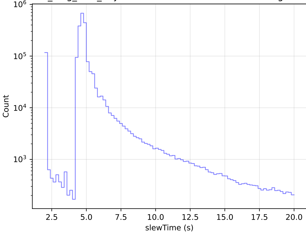
all_long_v3.4_10yrs All visits: Zoom Slew Time Histogram
