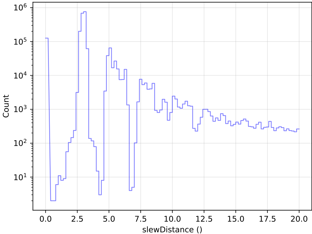
all_long_v3.4_10yrs All visits: Zoom Slew Distance Histogram
