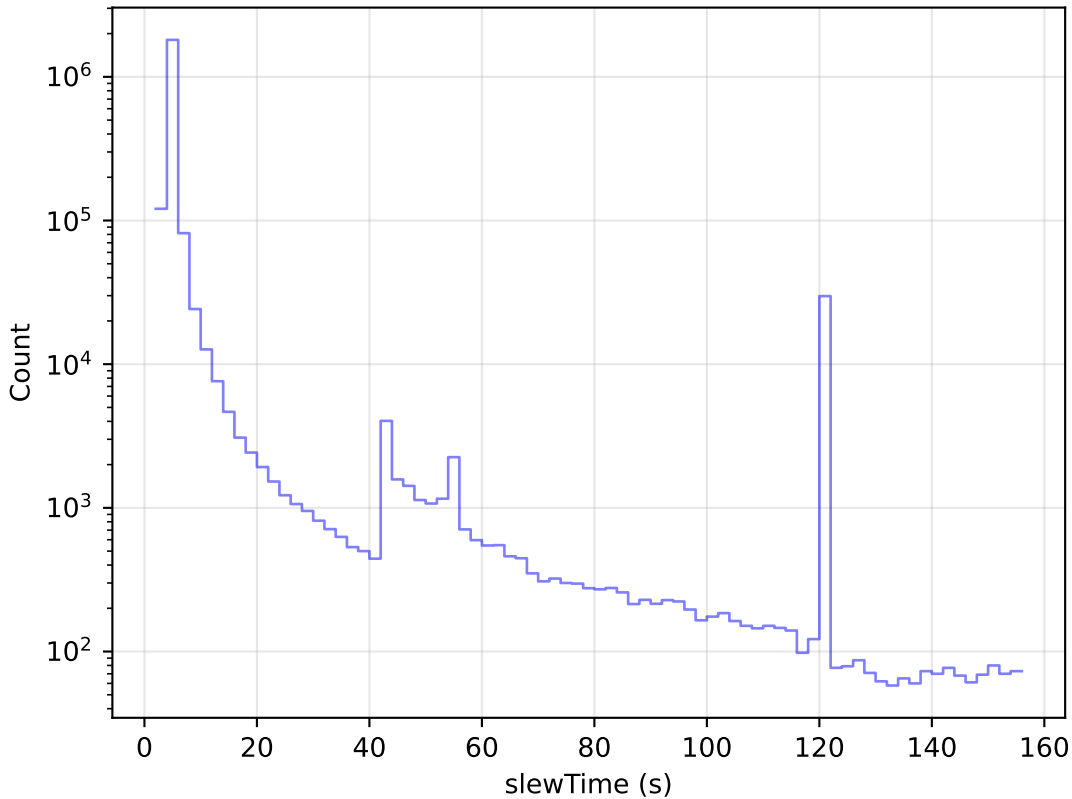
all_long_v3.4_10yrs All visits: Slew Time Histogram
