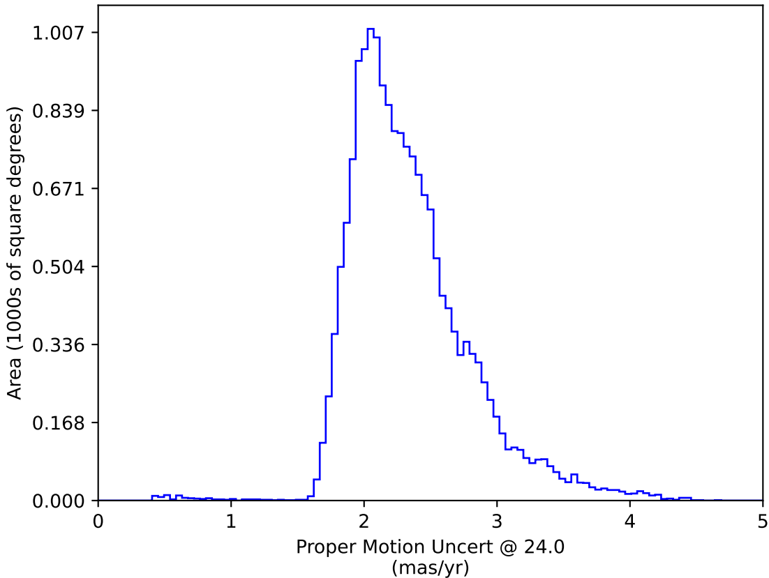
all_long_v3.4_10yrs WFD: Proper Motion Uncert @ 24.0
