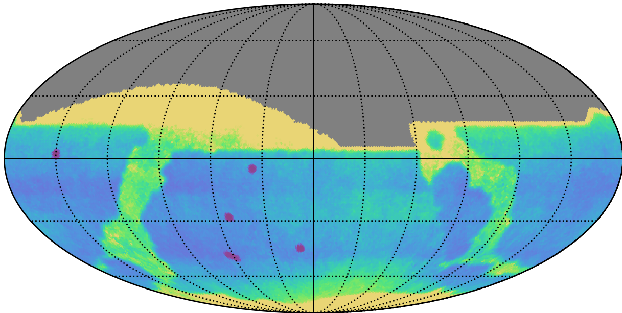
all_long_v3.4_10yrs All sky: Proper Motion Uncert @ 24.0
