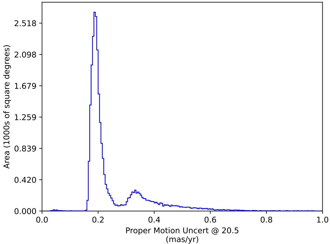
all_long_v3.4_10yrs All sky: Proper Motion Uncert @ 20.5
