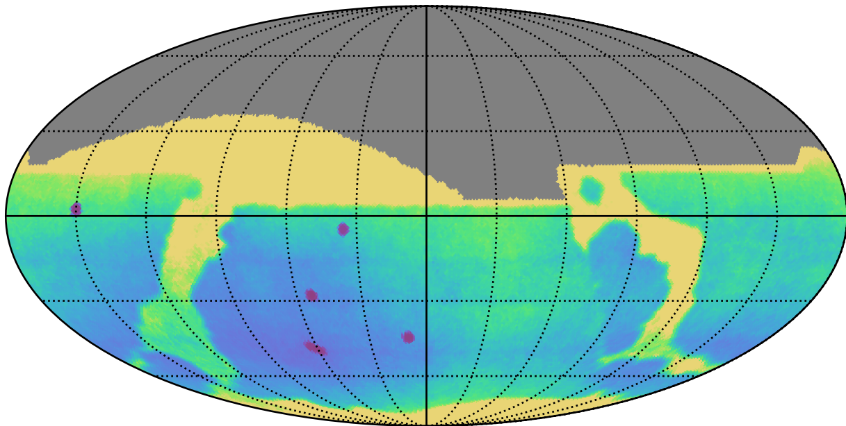
all_long_v3.4_10yrs All sky: Parallax Uncert @ 24.0
