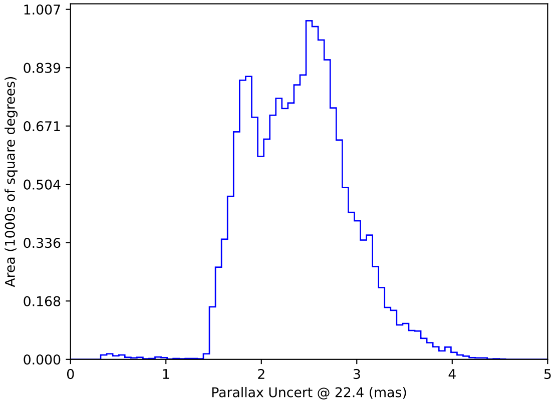
all_long_v3.4_10yrs WFD: Parallax Uncert @ 22.4
