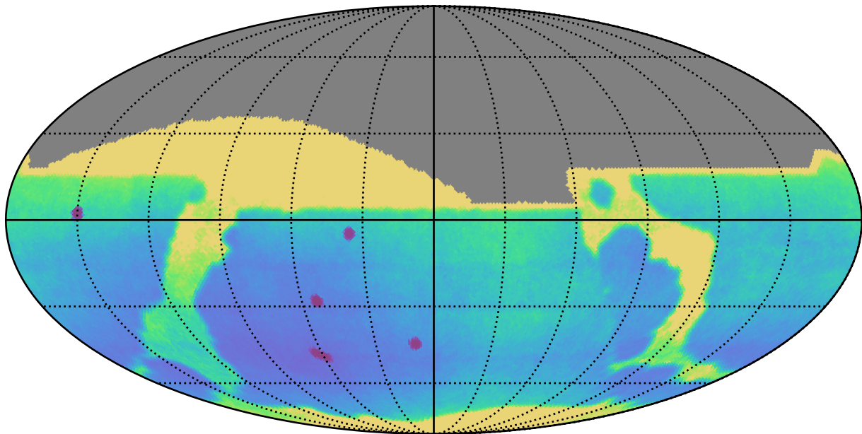
all_long_v3.4_10yrs All sky: Parallax Uncert @ 22.4
