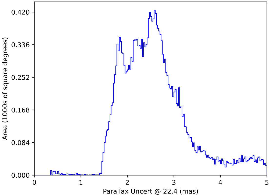
all_long_v3.4_10yrs All sky: Parallax Uncert @ 22.4
