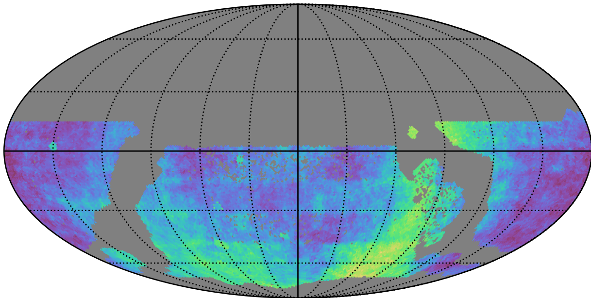
all_long_v3.4_10yrs WFD: Parallax Coverage @ 24.0
