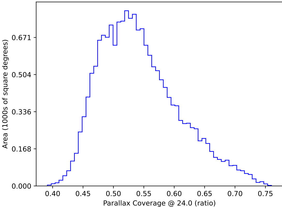
all_long_v3.4_10yrs WFD: Parallax Coverage @ 24.0
