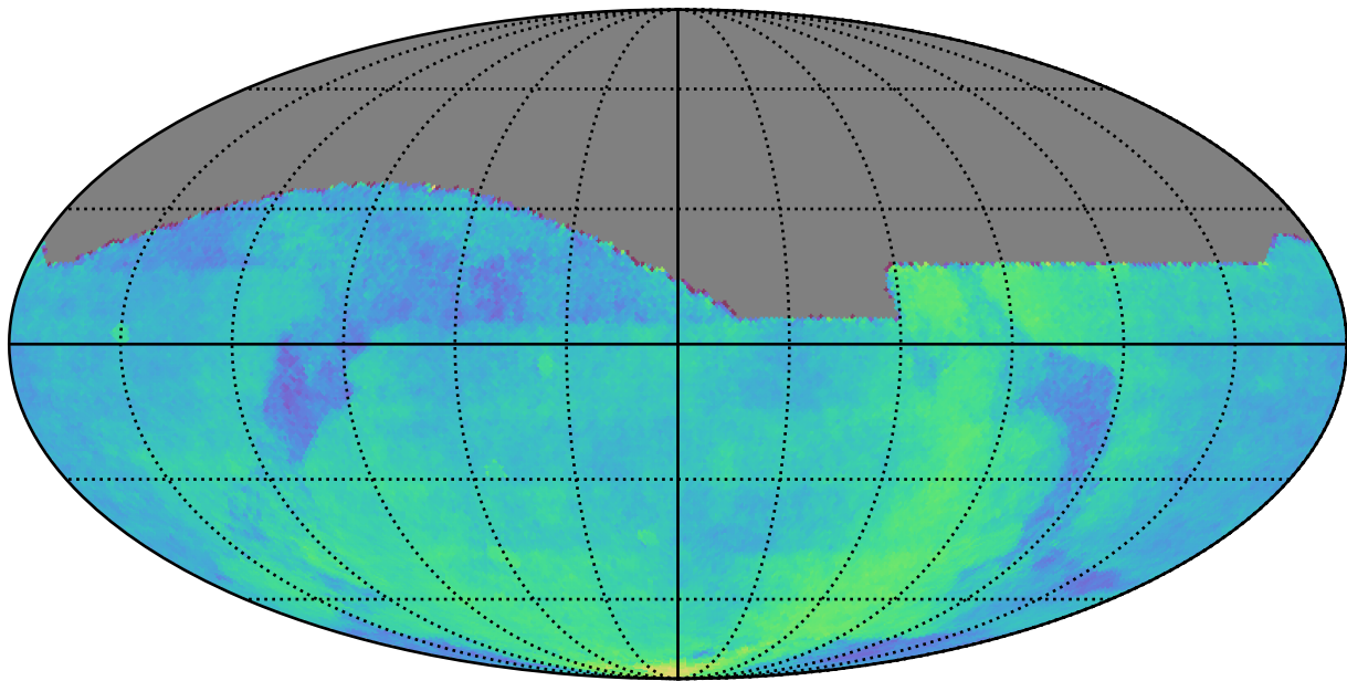
all_long_v3.4_10yrs All sky: Parallax Coverage @ 24.0
