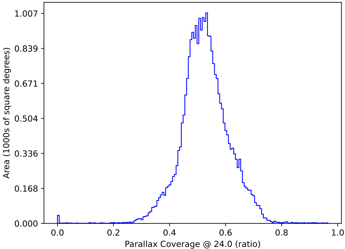
all_long_v3.4_10yrs All sky: Parallax Coverage @ 24.0
