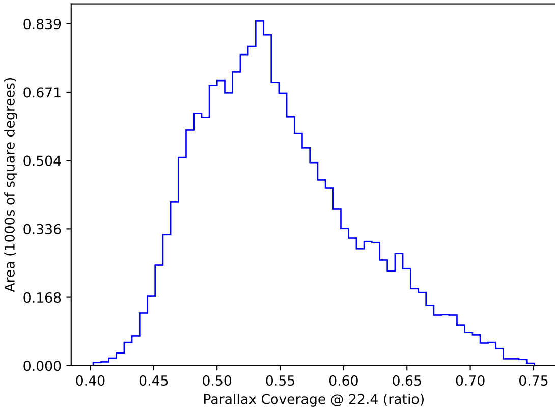
all_long_v3.4_10yrs WFD: Parallax Coverage @ 22.4
