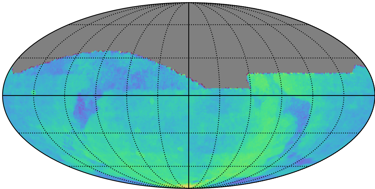
all_long_v3.4_10yrs All sky: Parallax Coverage @ 22.4
