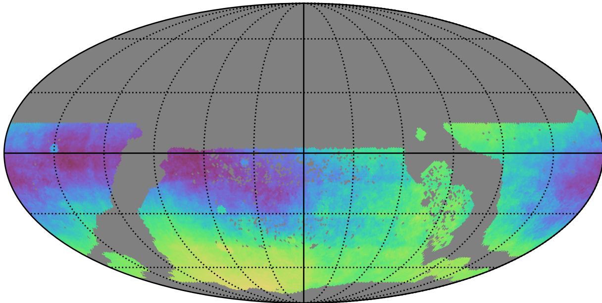
all_long_v3.4_10yrs WFD: Parallax-DCR degeneracy @ 24.0
