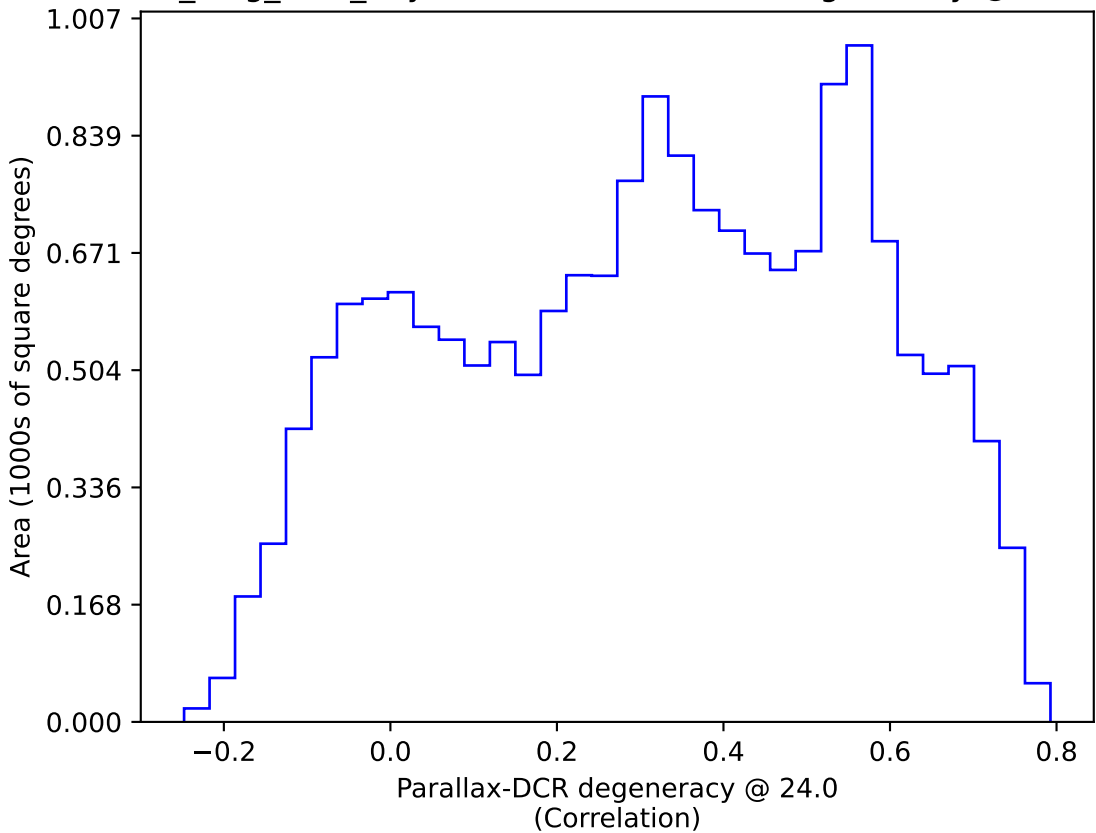
all_long_v3.4_10yrs WFD: Parallax-DCR degeneracy @ 24.0
