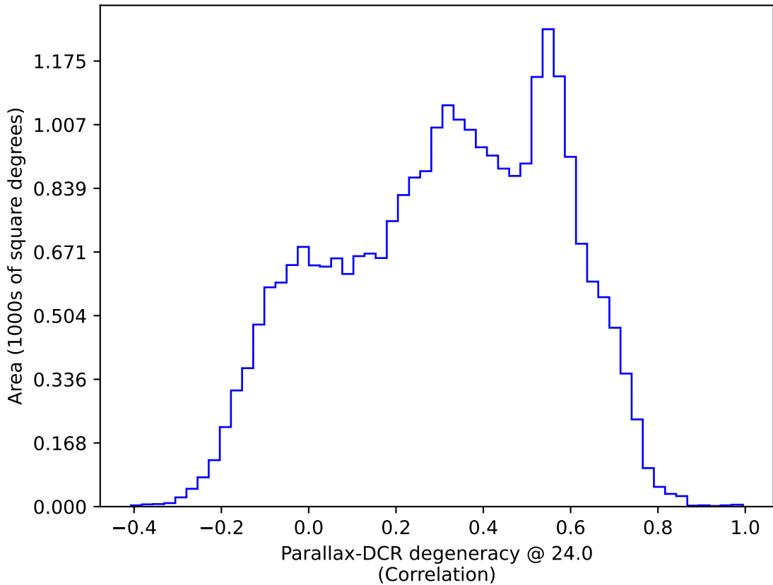
all_long_v3.4_10yrs All sky: Parallax-DCR degeneracy @ 24.0
