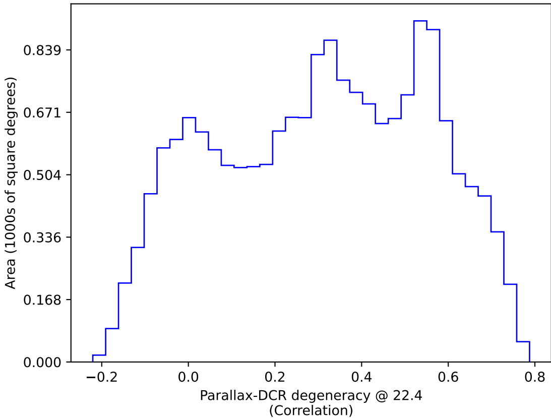
all_long_v3.4_10yrs WFD: Parallax-DCR degeneracy @ 22.4
