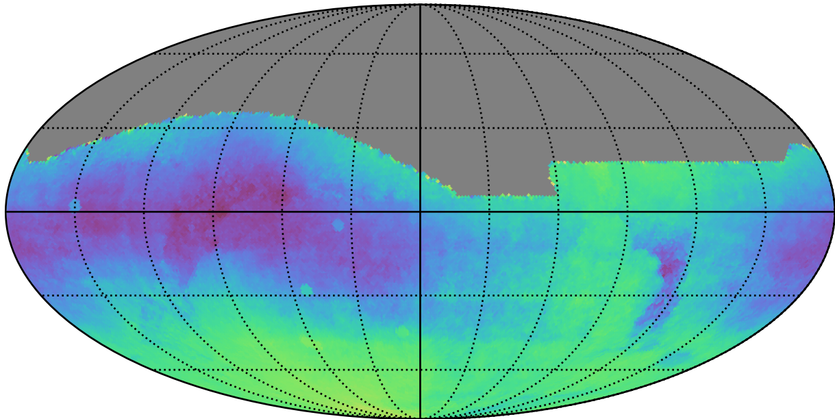
all_long_v3.4_10yrs All sky: Parallax-DCR degeneracy @ 22.4
