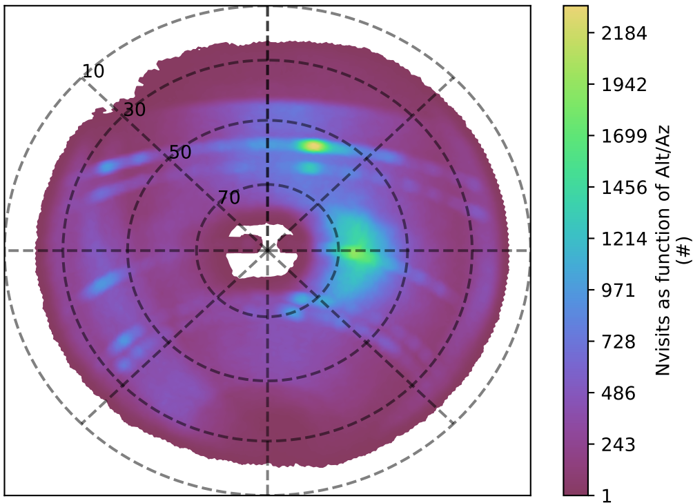
all_long_v3.4_10yrs z band: Nvisits as function of Alt/Az
