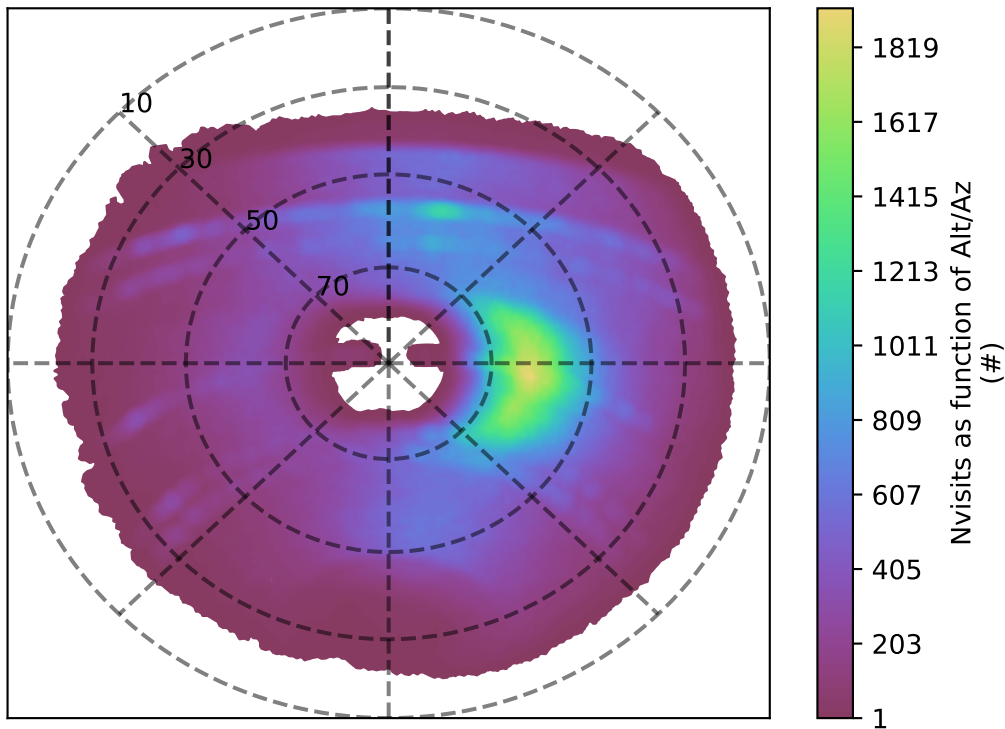
all_long_v3.4_10yrs y band: Nvisits as function of Alt/Az
