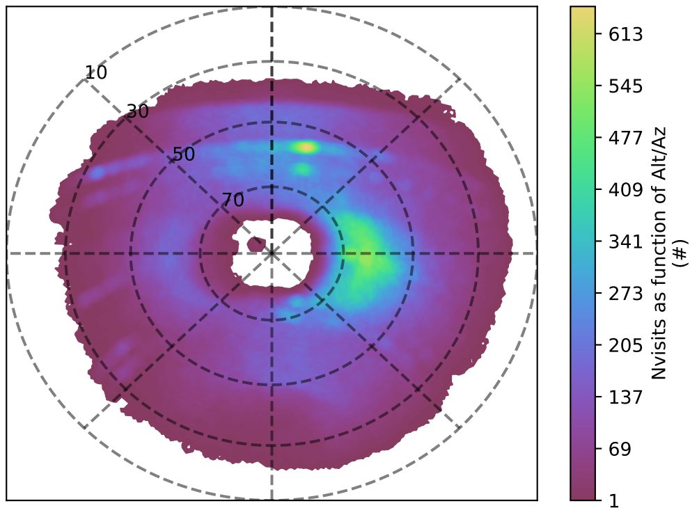
all_long_v3.4_10yrs u band: Nvisits as function of Alt/Az
