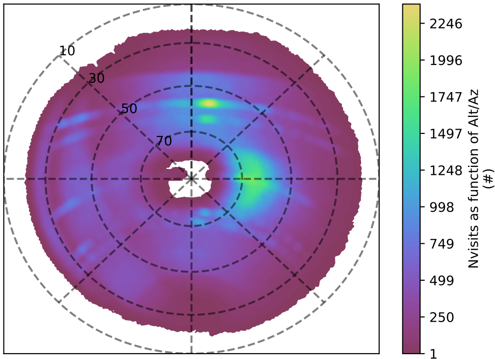
all_long_v3.4_10yrs r band: Nvisits as function of Alt/Az
