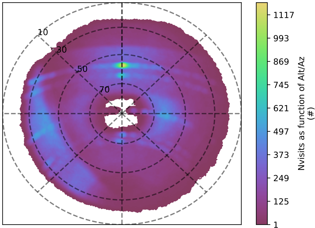
all_long_v3.4_10yrs g band: Nvisits as function of Alt/Az
