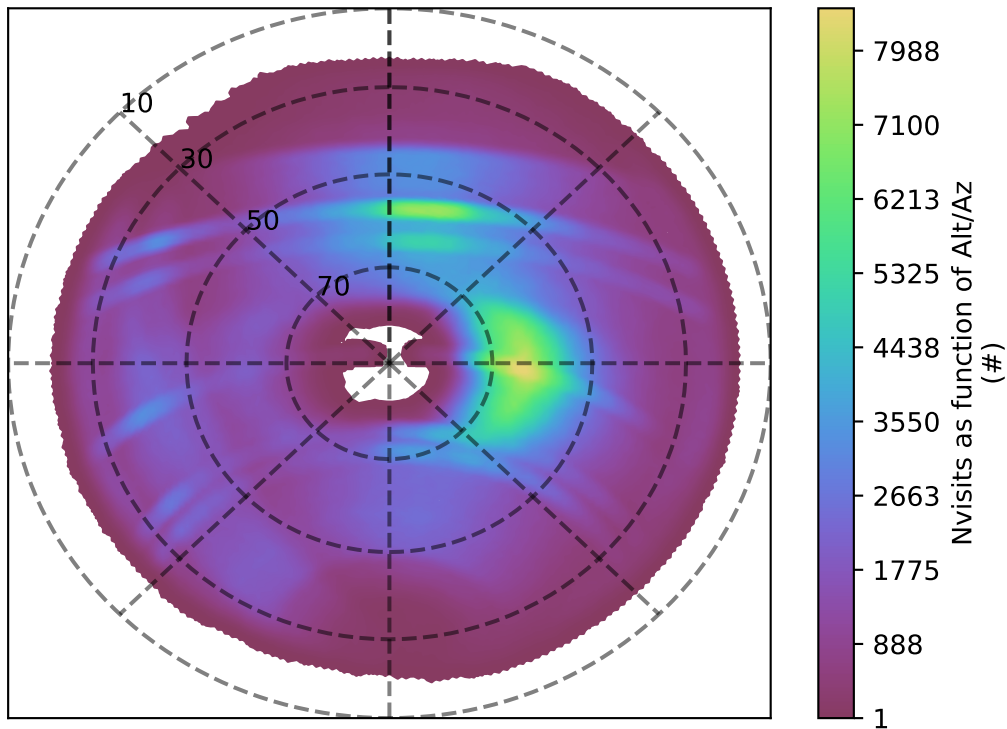
all_long_v3.4_10yrs all bands: Nvisits as function of Alt/Az
