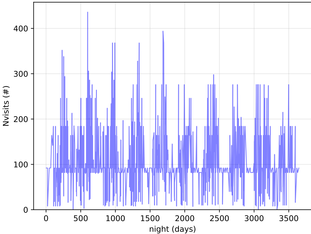
all_long_v3.4_10yrs DDF: Nvisits
