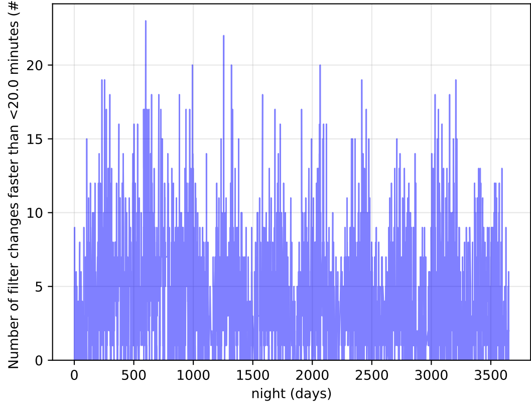
all_long_v3.4_10yrs Per Night: Number of filter changes faster than <20.0 minutes
