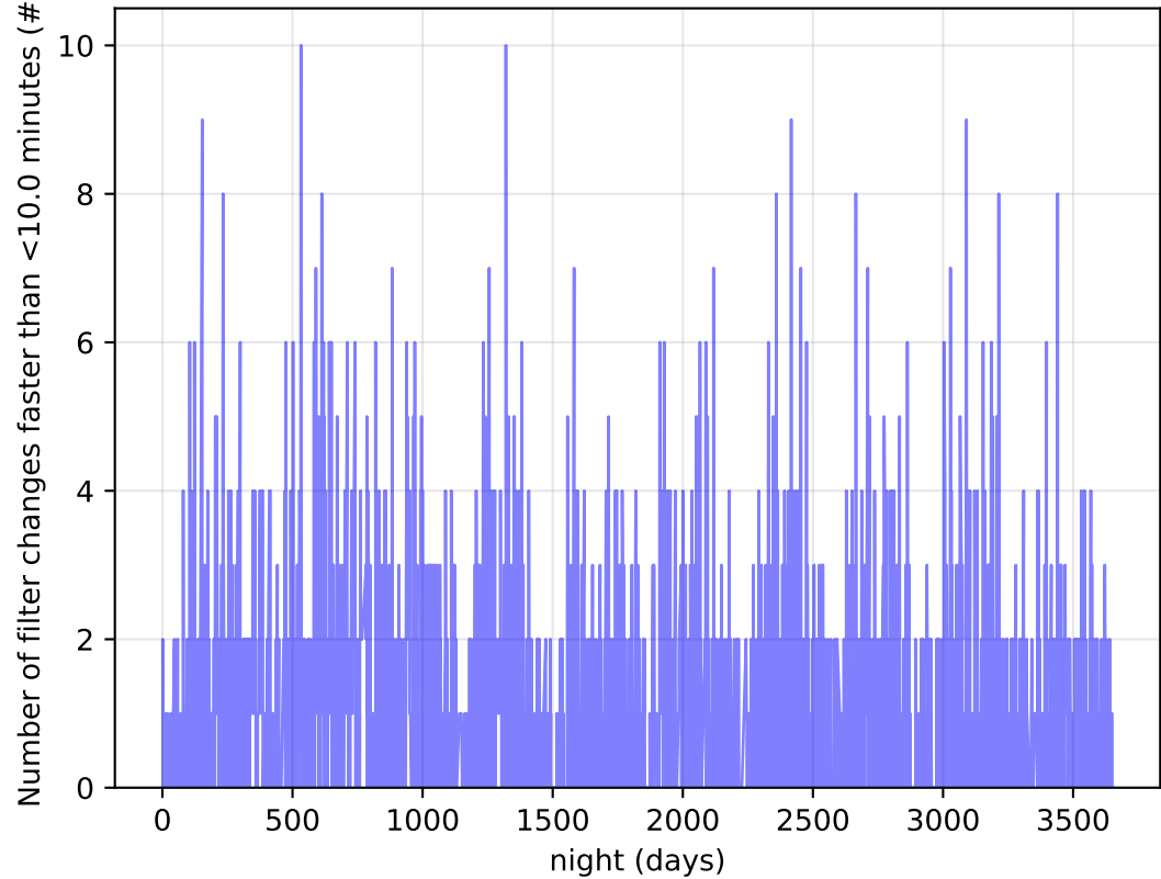
all_long_v3.4_10yrs Per Night: Number of filter changes faster than <10.0 minutes
