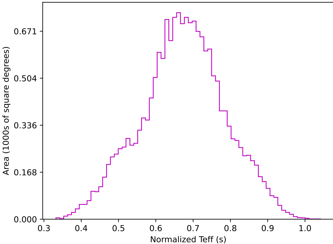
all_long_v3.4_10yrs WFD z band: Normalized Teff
