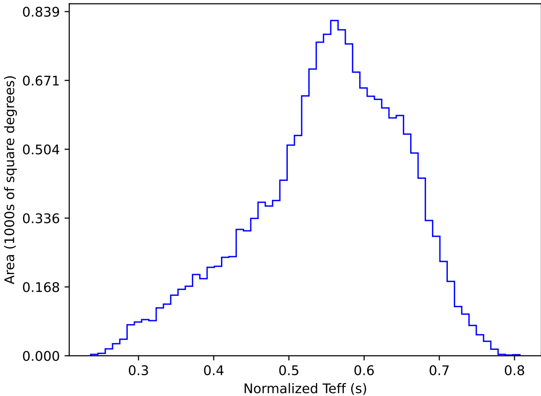
all_long_v3.4_10yrs WFD y band: Normalized Teff
