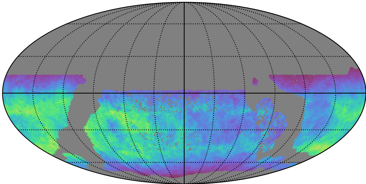
all_long_v3.4_10yrs WFD u band: Normalized Teff
