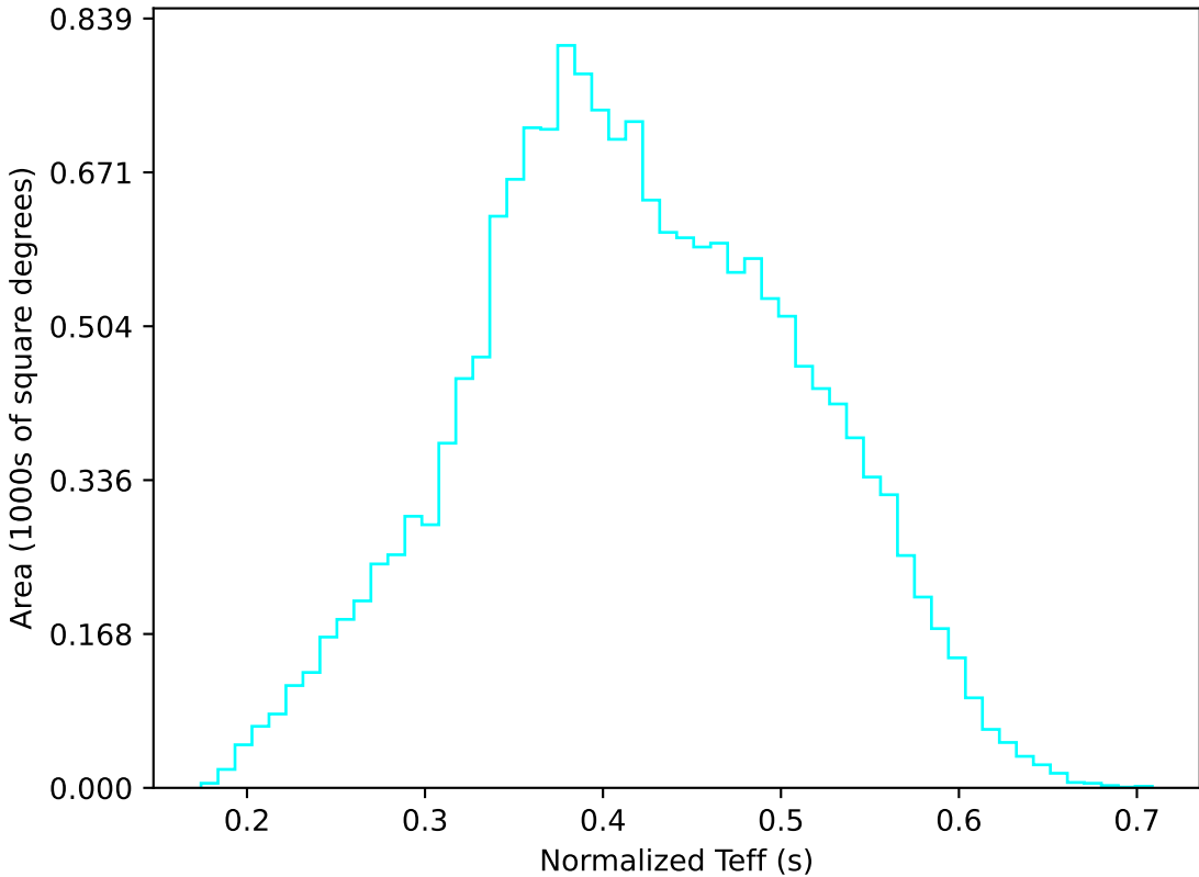
all_long_v3.4_10yrs WFD u band: Normalized Teff
