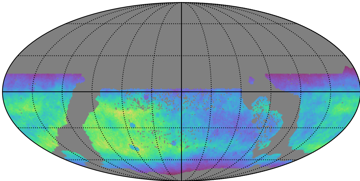
all_long_v3.4_10yrs WFD r band: Normalized Teff
