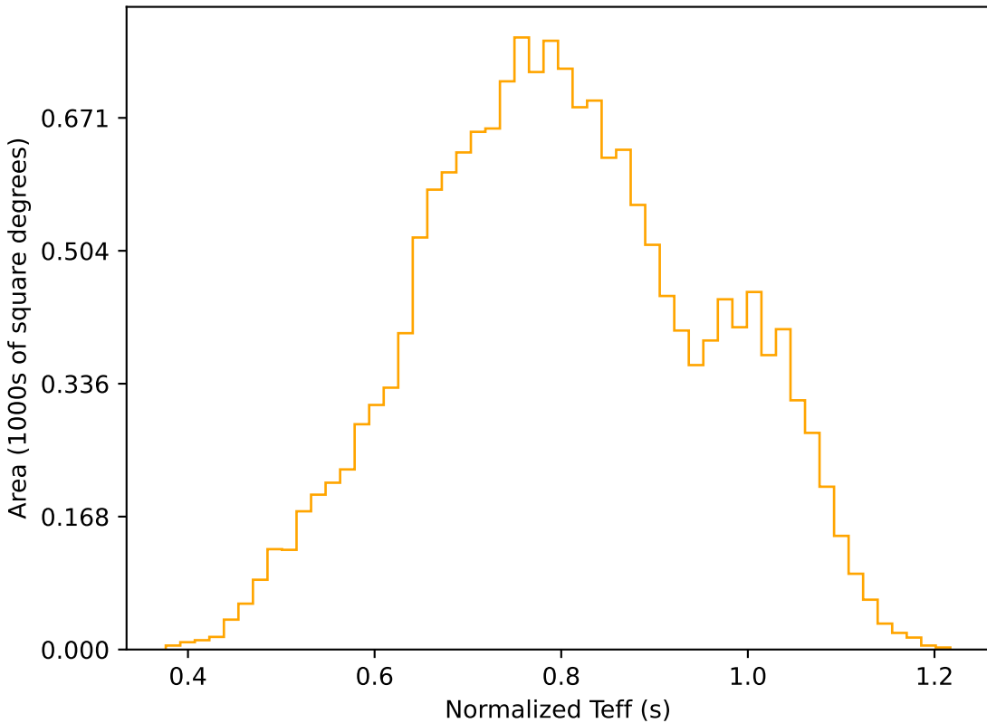
all_long_v3.4_10yrs WFD r band: Normalized Teff
