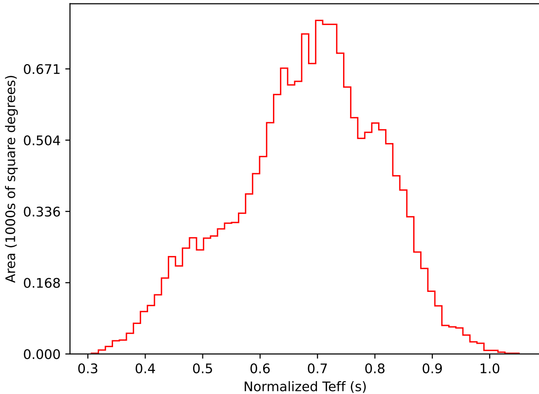
all_long_v3.4_10yrs WFD i band: Normalized Teff
