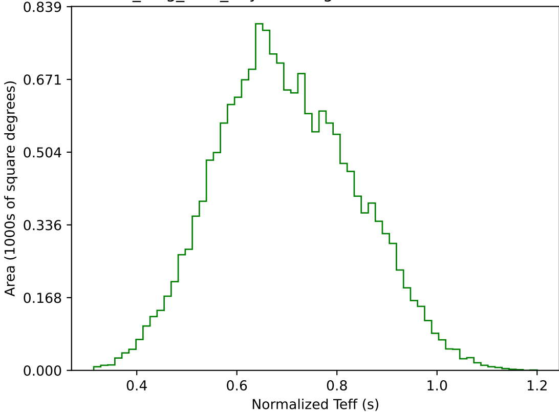
all_long_v3.4_10yrs WFD g band: Normalized Teff
