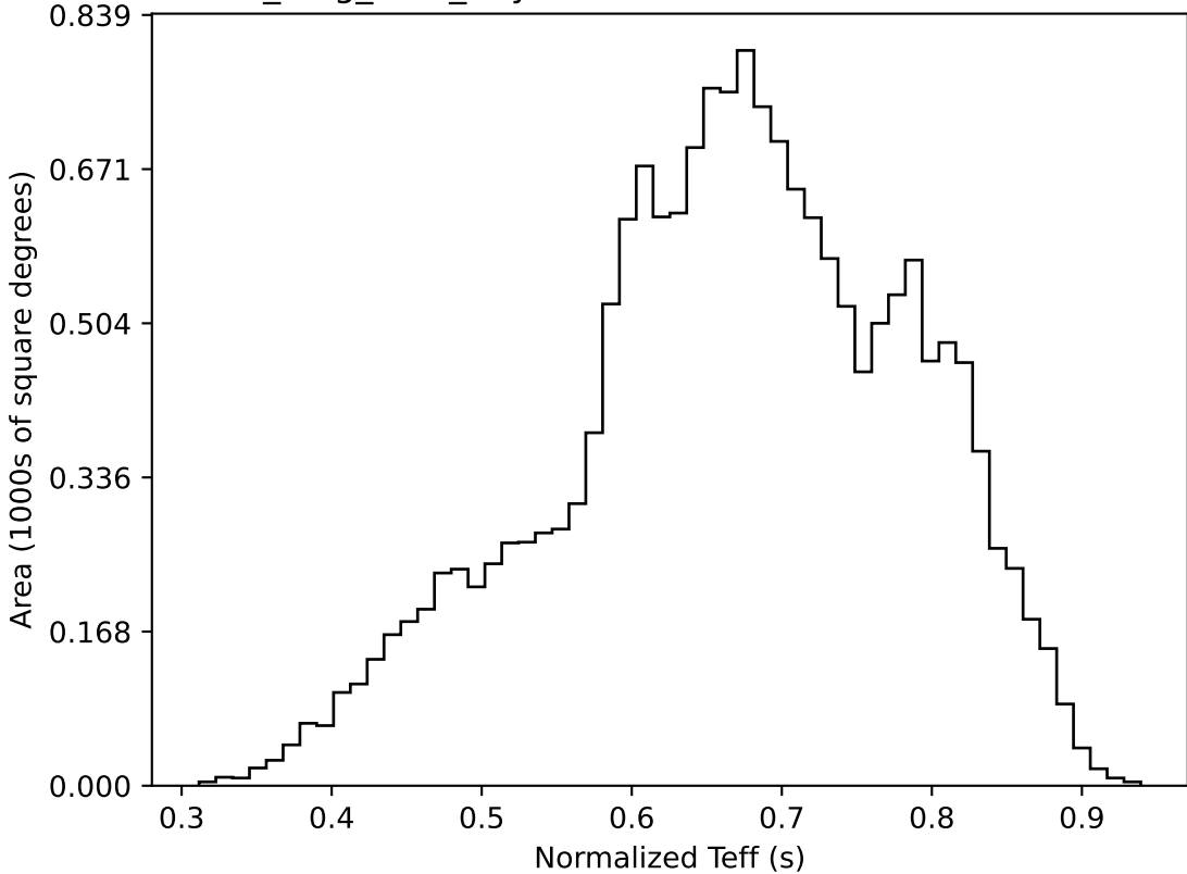
all_long_v3.4_10yrs WFD all bands: Normalized Teff
