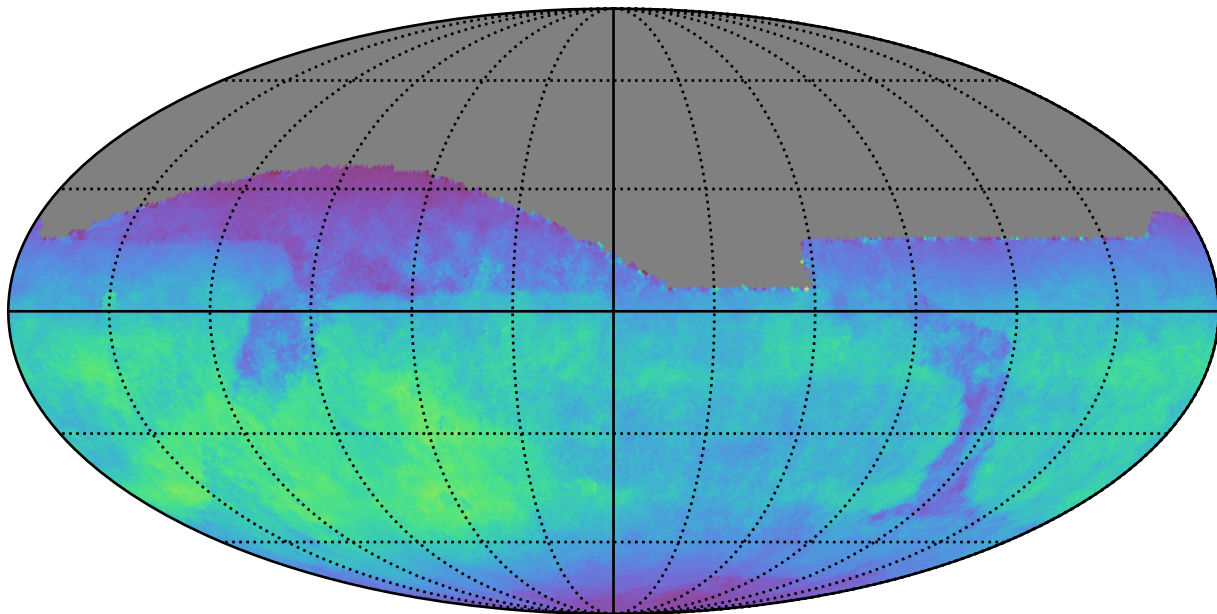
all_long_v3.4_10yrs All sky z band: Normalized Teff
