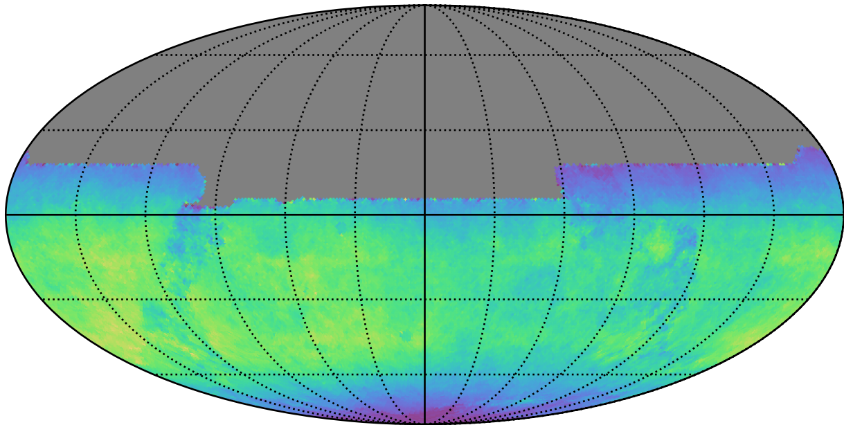
all_long_v3.4_10yrs All sky y band: Normalized Teff
