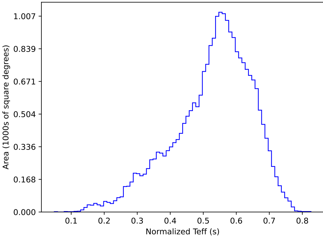
all_long_v3.4_10yrs All sky y band: Normalized Teff
